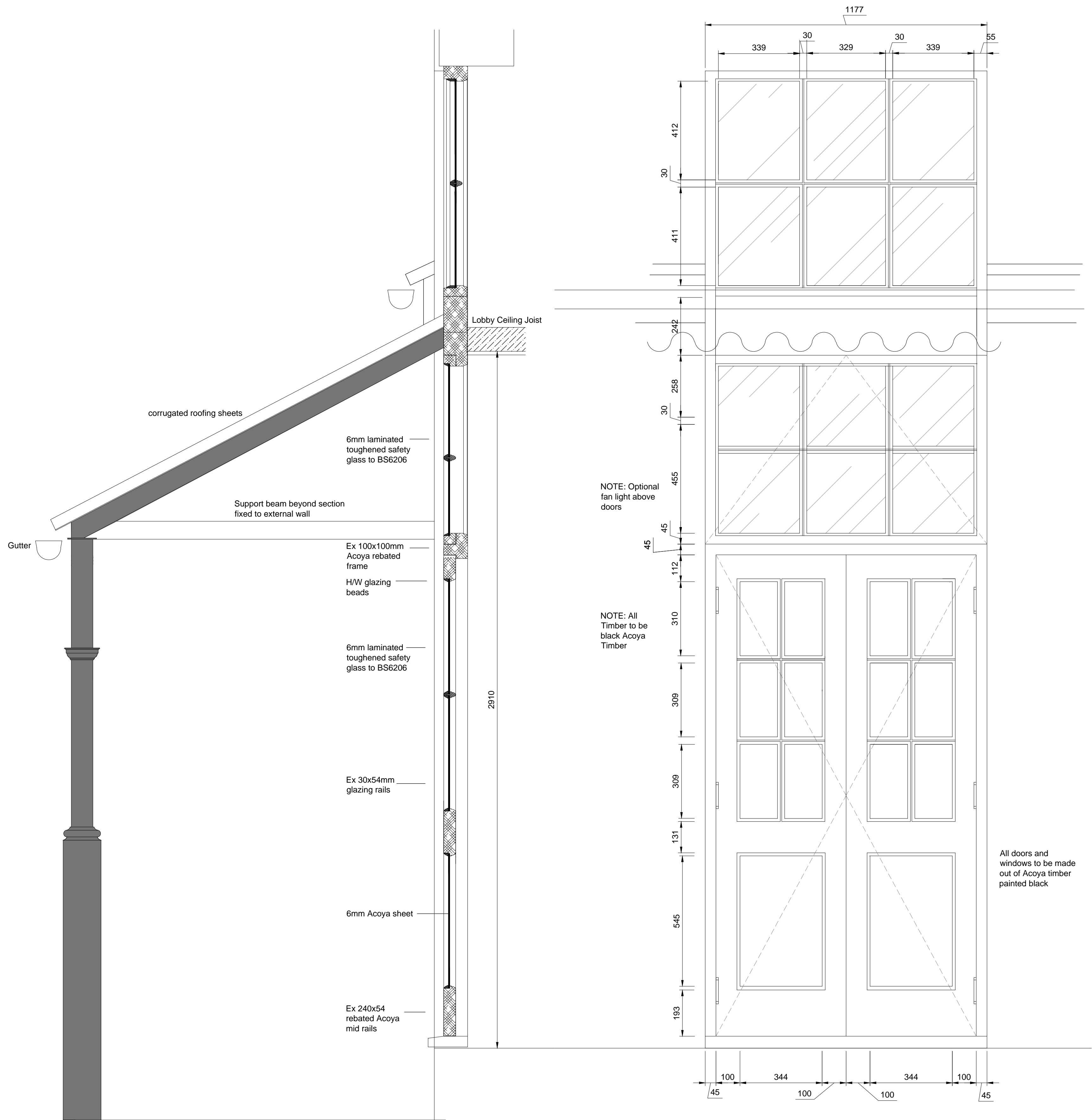
Full Height Entrance Door Detail Scale 1:10
